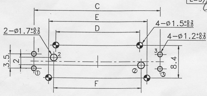
P.C.B. MOUNTING HOLE DETAIL
