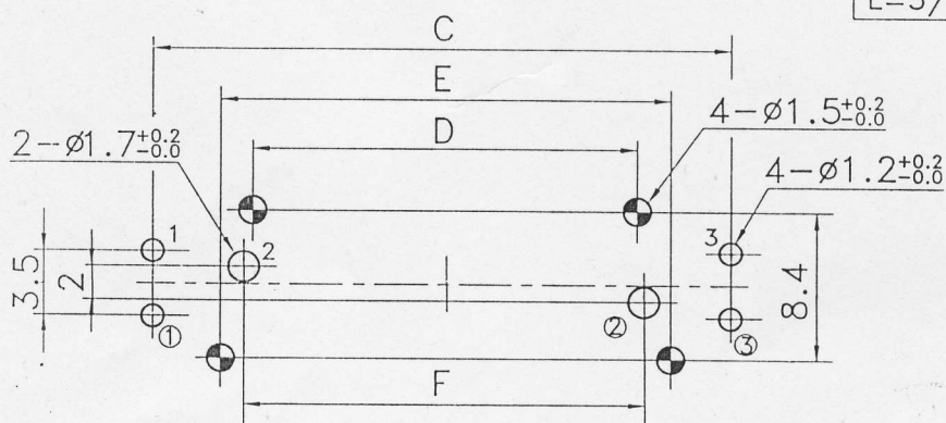
P.C.B. MOUNTING HOLE DETAIL
