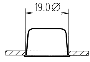
MOUNTING VM-100 WITH 8''M-60/N
