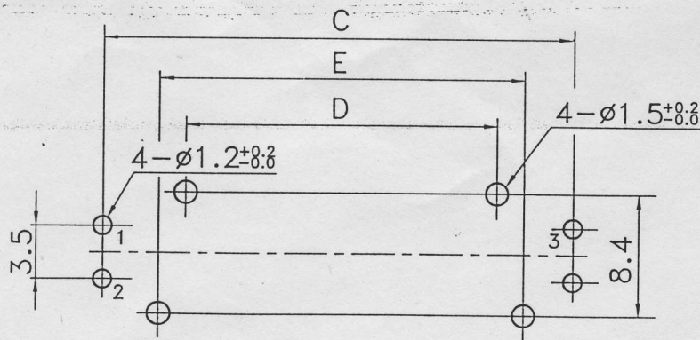
P.C.B. MOUNTING HOLE DETAIL
